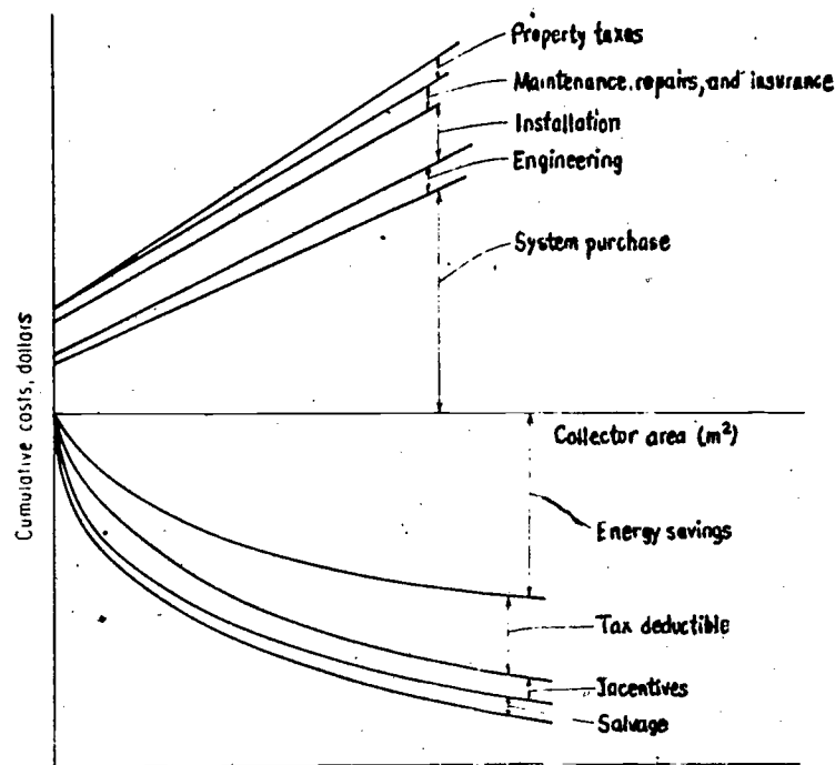
Fixed and variable cost components. (Fixed costs are the differences in the intercepts of the upper arrows)
