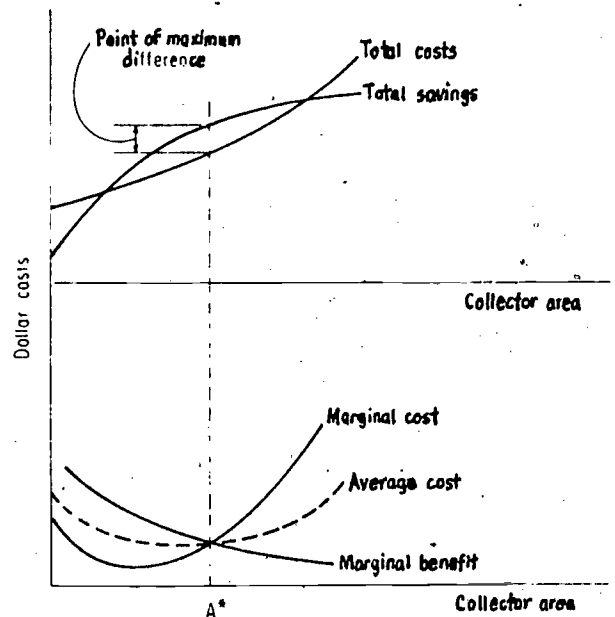
The relationship of total, marginal, and average costs of a solar energy system
